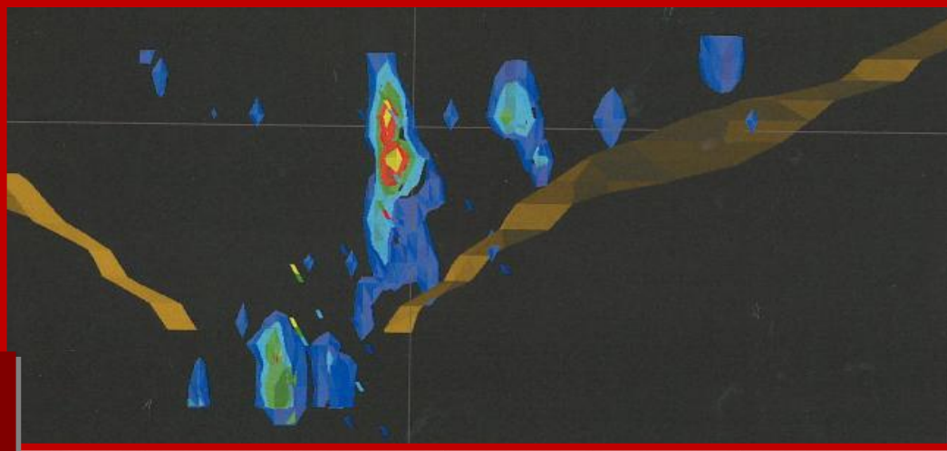
Sleeper Pit area with Au system grade shells, topography, and geology contacts (section 8600N looking north).
