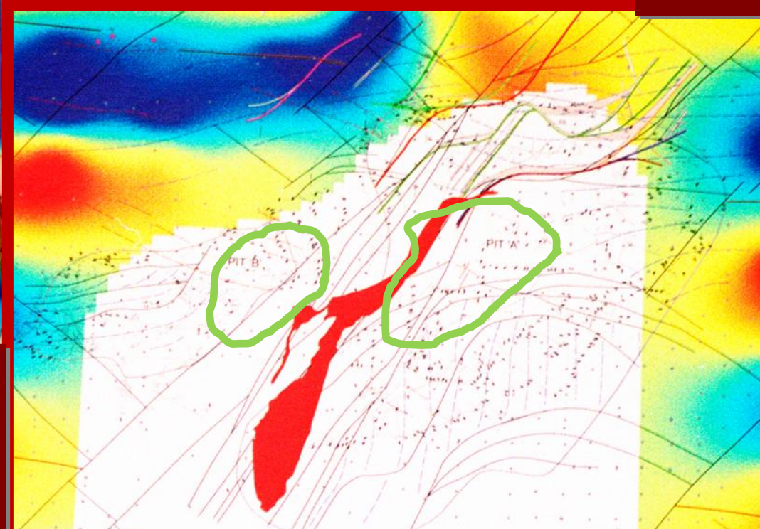
The OreFull Mineral Texture Atlases Volume 48 – 2 : North Queensland Epithermals WIRRALIE - Regional Magnetics Shaded RTP on Dipole Dipole Resistivity. Pits A and B in green and possible targets in red (left side). Resistivity is on the right side. Data with permission from Delta Gold and initially generated by Dr. Greg Partington and Team .
