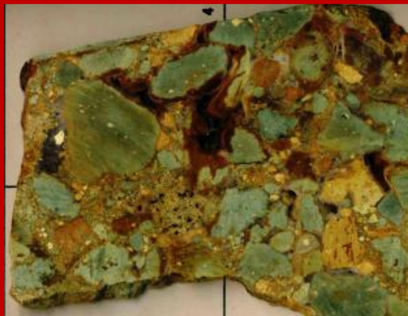
The OreFull Mineral Texture Atlases Volume 48 – 5 : North Queensland Epithermals Yandan - Discovery Outcrops Lone Sister Breccias and “sinters” proximal to the Twin Hills Epithermal Deposit © James Stewart 2013 www.orefullmineraltextures.com
